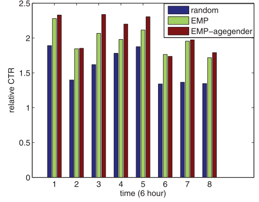
Fig. 11. CTR comparison in bucket test at eight consecutive 6-hour time slots during 2 days, where relative CTR is computed by scaling the absolute CTR by a constant factor.
