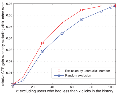
Fig. 8. Relative precision gain when training with data after excluding some nonclick events over training with data excluding only click-other events (using EMP-kmeans ).
