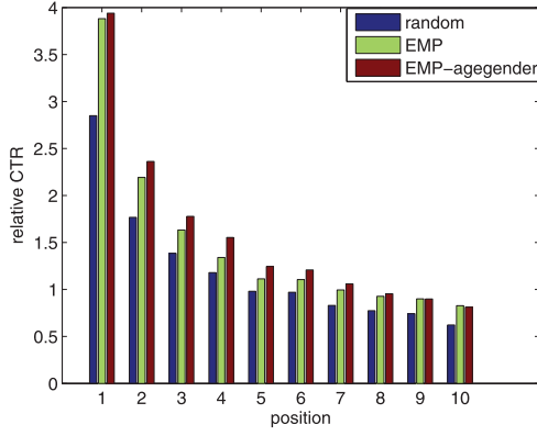
Fig. 10. CTR comparison in bucket test at different positions, where relative CTR is computed by scaling the absolute CTR by a constant factor.
