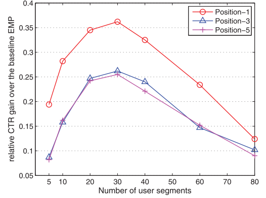
Fig. 7. Relative precision gain of EMP-kmeans over the baseline against varying number of user segments.
