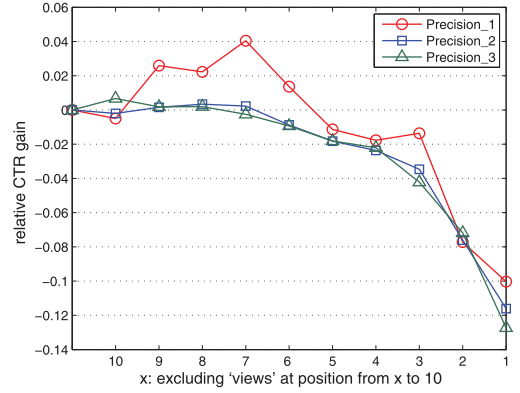
Fig. 9. Relative precision gains by removing view samples at the positions close to bottom.
