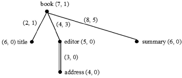
Fig. 14. Sample weighted tree pattern.
