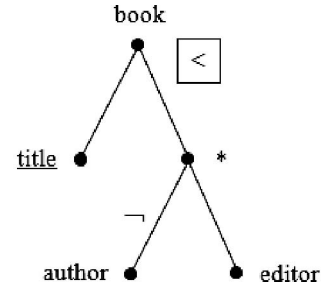
Fig. 9. Sample extended tree pattern.
