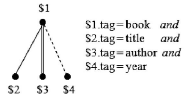
Fig. 3. Sample generalized tree pattern.
