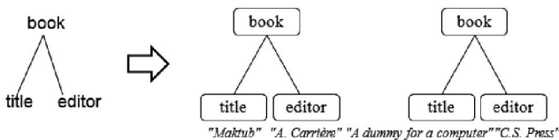
Fig. 12. Sample holistic matching.
