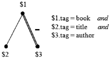
Fig. 4. Sample annotated pattern tree.
