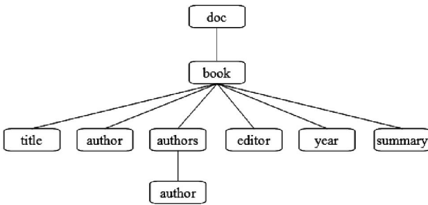
Fig. 13. Sample DataGuide.
