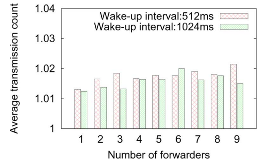
Fig. 10. Average transmission count of the successfully delivered packet.
