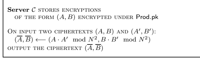
Fig. 5. Add. Given two ciphertexts (A, B) and (A', B') encrypted under \text{Prod.pk} , it computes an encryption of the sum of the underlying plaintexts.
