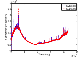
Fig. 8. Piecewise linear cost: Total # sessions needed with a 15 sec ICC pulse width - Operational trace, 15 sec deadline for VoD
