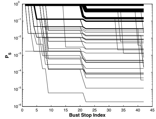
Fig. 10. Evaluating P_S for a number of trips conducted on route 150.
