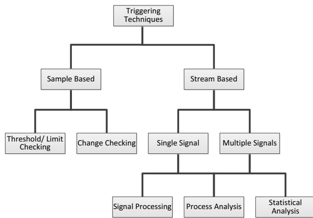
Fig. 3. Event detection techniques.
