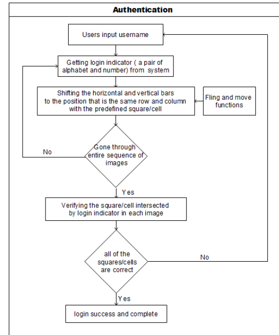
Fig. 10. The flowchart of authentication phase in PassMatrix.
