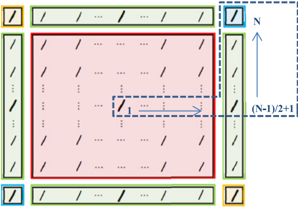
Fig. 2. Schematic illustration of a large array divided into subarrays based on the element characteristics. The simulated elements in each subarray, used to represent the field distribution of all elements in the subarray, are marked in bold. The numbers 1, (N-1)/2+1 and N , corresponds to the element positions used in Fig. 4, and the arrows indicate the directions of increasing element position.
