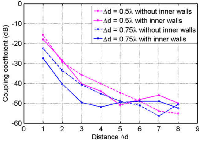
Fig. 6. Coupling coefficient between an active element located at the edge of the center row in a 9 \times 9 array antenna to the other elements in the same row.
