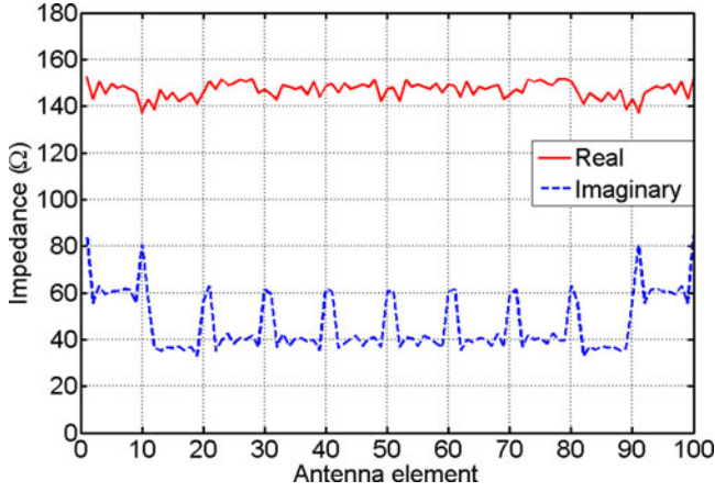
Fig. 1. Impedance characteristics for a uniformly excited 10 \times 10 ground-plane backed dipole array antenna as function of element position. The used interelement spacing was half a wavelength.
