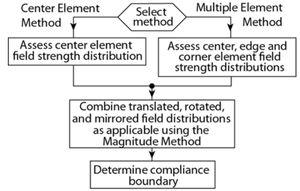
Fig. 3. Flowchart of the proposed approximate methods for RF EMF compliance assessments of large array antennas.
